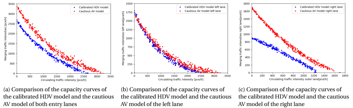
Figure 5.1: Comparison of the capacity curves of the calibrated HDV model and the cautious AV model for the minor roundabout entrance. The blue dots indicate the calibrated HDV model results, and the red dots represent the simulation data of the cautious AV model.
