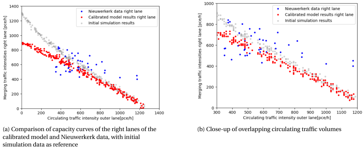
Figure 4.20: Comparison of the capacity curves of the calibrated simulation and the Nieuwerkerk data with the initial simulation data as a reference, for the right entry lane of the minor roundabout entrance. The red dots represent the calibrated simulation results, the blue dots represent the Nieuwerkerk data, and the transparent grey dots represent the initial simulation data.
