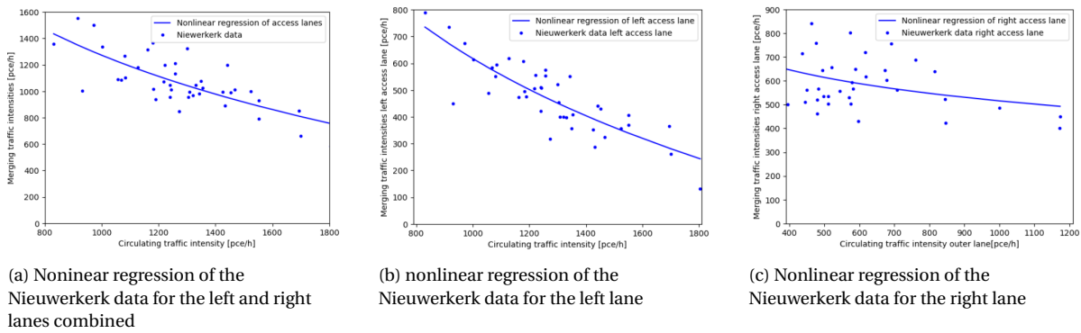
Figure 4.5: Nonlinear regression of various lane configurations of the Nieuwerkerk data
