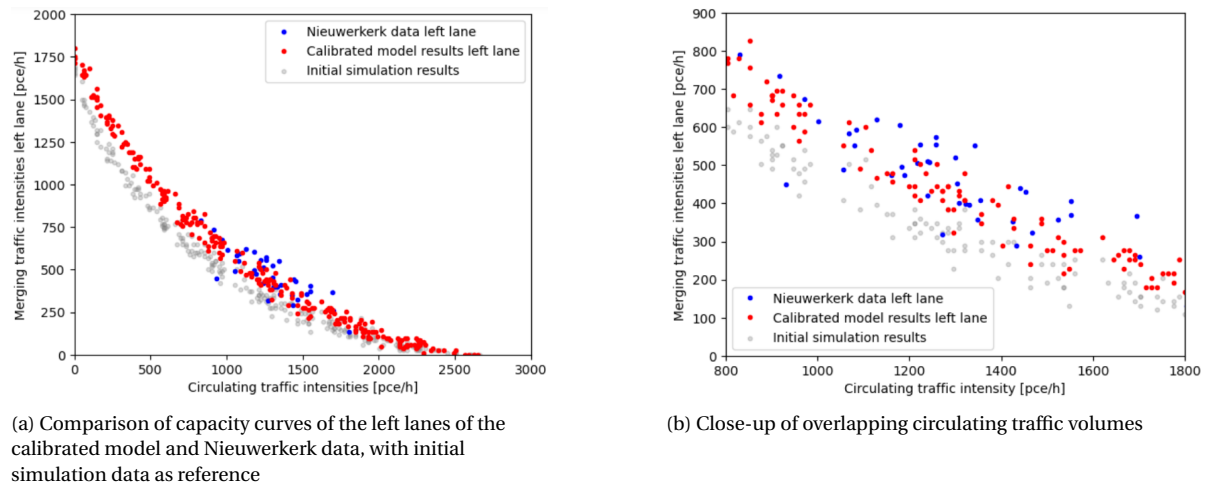
Figure 4.19: Comparison of the capacity curves of the calibrated simulation and the Nieuwerkerk data with the initial simulation data as a reference, for the left entry lane of the minor roundabout entrance. The red dots represent the calibrated simulation results, the blue dots represent the Nieuwerkerk data, and the transparent grey dots represent the initial simulation data.
