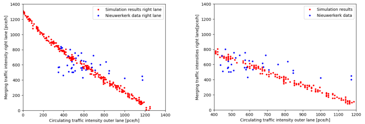
(a) Comparison of capacity curves for the right lane of the simulation model and Nieuwerkerk data. Once again, the red dots indicate the simulation data, and the blue dots represent the Nieuwerkerk data.
