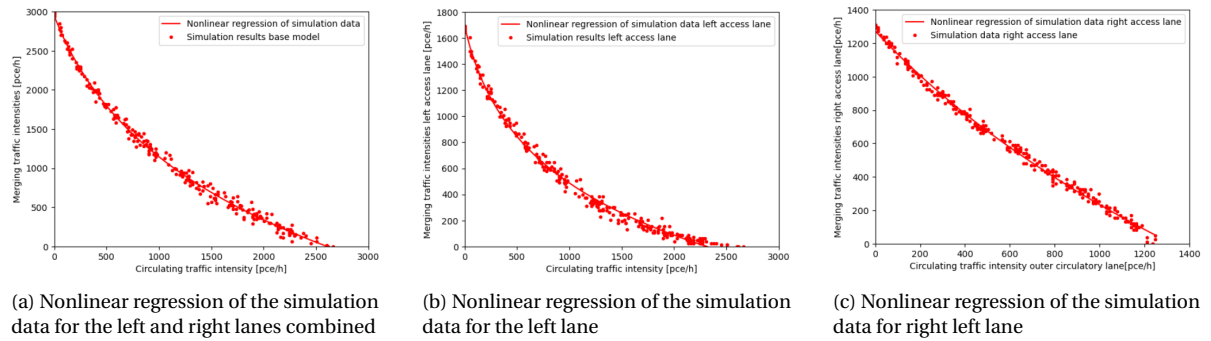
Figure 4.7: Nonlinear regression of various lane configurations of the simulation data
