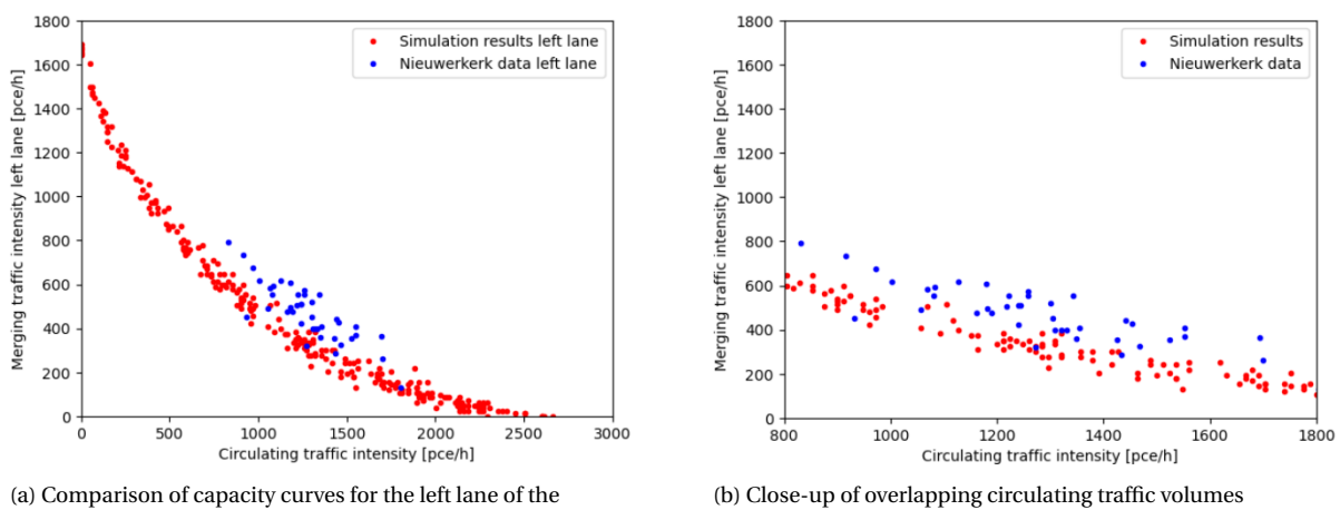
Figure 4.2: Comparison of the capacity curves of the simulation and Nieuwerkerk data for the left entry lanes of the minor roundabout entrance. Once again, the red dots indicate the simulation data, and the blue dots represent the Nieuwerkerk data.
