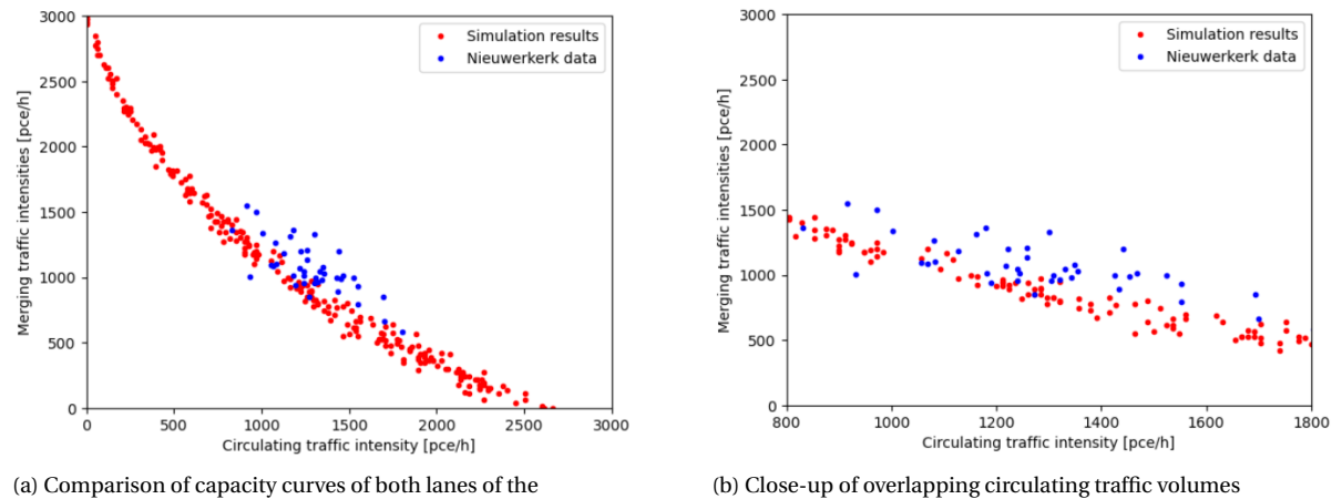
Figure 4.1: Comparison of the capacity curves of the simulation and Nieuwerkerk data for both entry lanes of the minor roundabout entrance. The red dots indicate the simulation data and the blue dots represent the Nieuwerkerk data.
