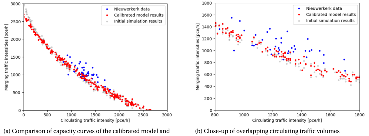
Figure 4.18: Comparison of the capacity curves of the calibrated simulation and the Nieuwerkerk data with the initial simulation data as a reference, for both entry lanes of the minor roundabout entrance. The red dots represent the calibrated simulation results, the blue dots represent the Nieuwerkerk data, and the transparent grey dots represent the initial simulation data.
