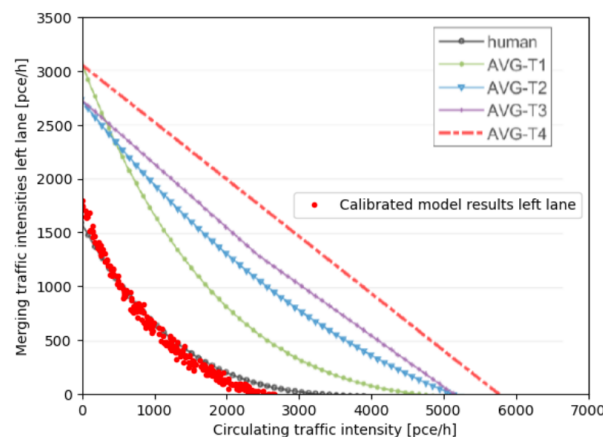
Figure 4.21: Comparison of simulation outcomes with theoretical 'human' model of Fortuijn and Salomons (Fortuijn and Salomons, 2020). The red dots indicate the calibrated model and are plotted over the theoretical curves of Fortuijn and Salomons.
