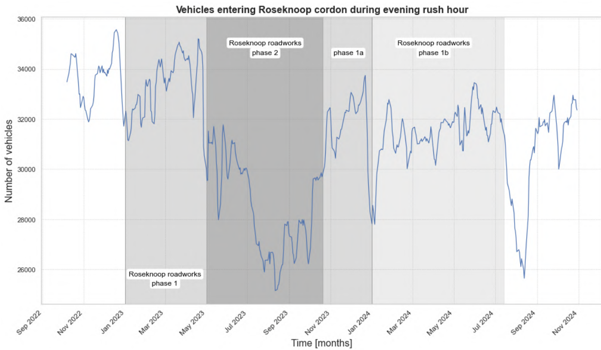
Figure 5.7: Number of vehicles entering Roseknoop cordon for evening peak period between 3 and 5PM (5 day rolling average).
