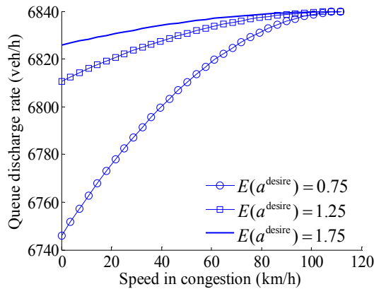
10 a) Sensitivity of the analytical model 11 to the mathematic expectation of 12 desired accelerations.
