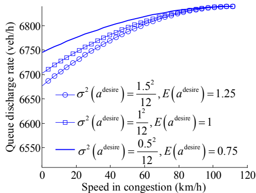
16 c) Comparisons of impacts on queue 17 discharge rates between the 18 mathematical expectation and the 19 standard deviations of desired 20 accelerations.
