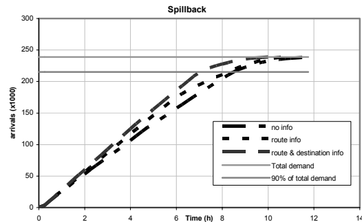
Fig. 4: Arrivals outside evacuation area in time in different information scenarios; results from a simulator with spillback
