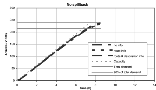
Fig. 3: Arrivals outside evacuation area in time in different information scenarios; results from a simulator without spillback. Also the maximum outflow is indicated
